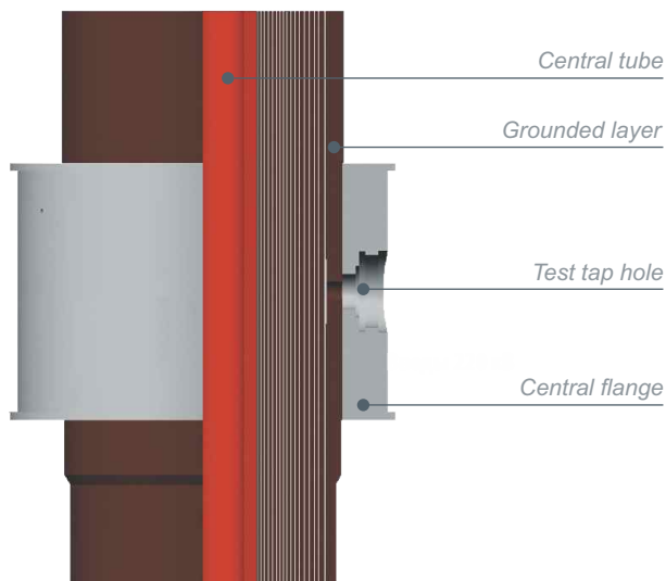
Fig. 3. Internal RIP-insulation
