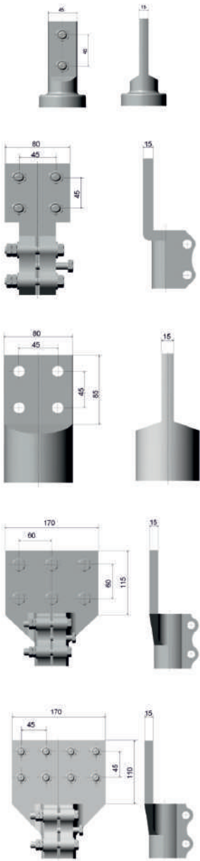
Fig. 14 Contact terminals
