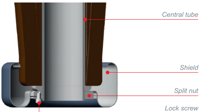
Fig. 11 Shield secured with screws
